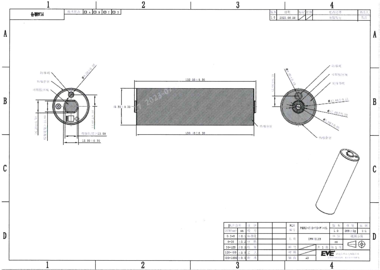
附图一：IFR40135 图纸 (Attachment I: IFR40135 drawing)
