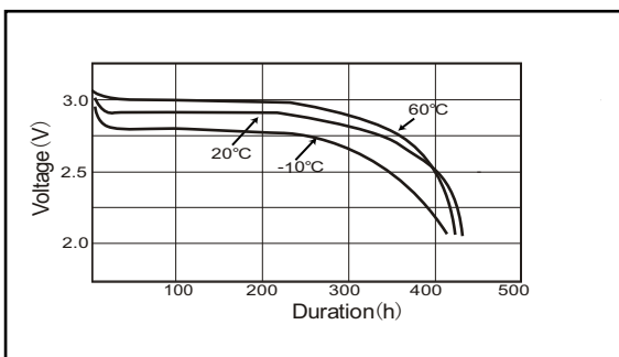
Temperature characteristics Load 15KΩ
