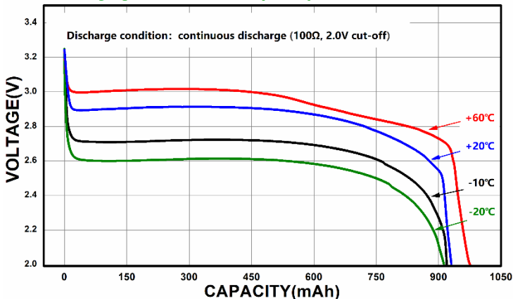
Discharging Characteristics by Temperature
