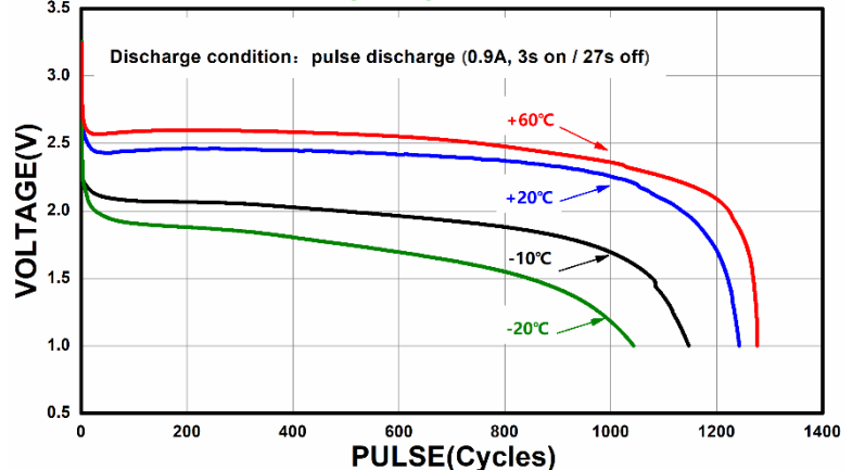
Pulse Characteristics by Temperature
